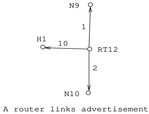
Figure 4: Individual link state components
